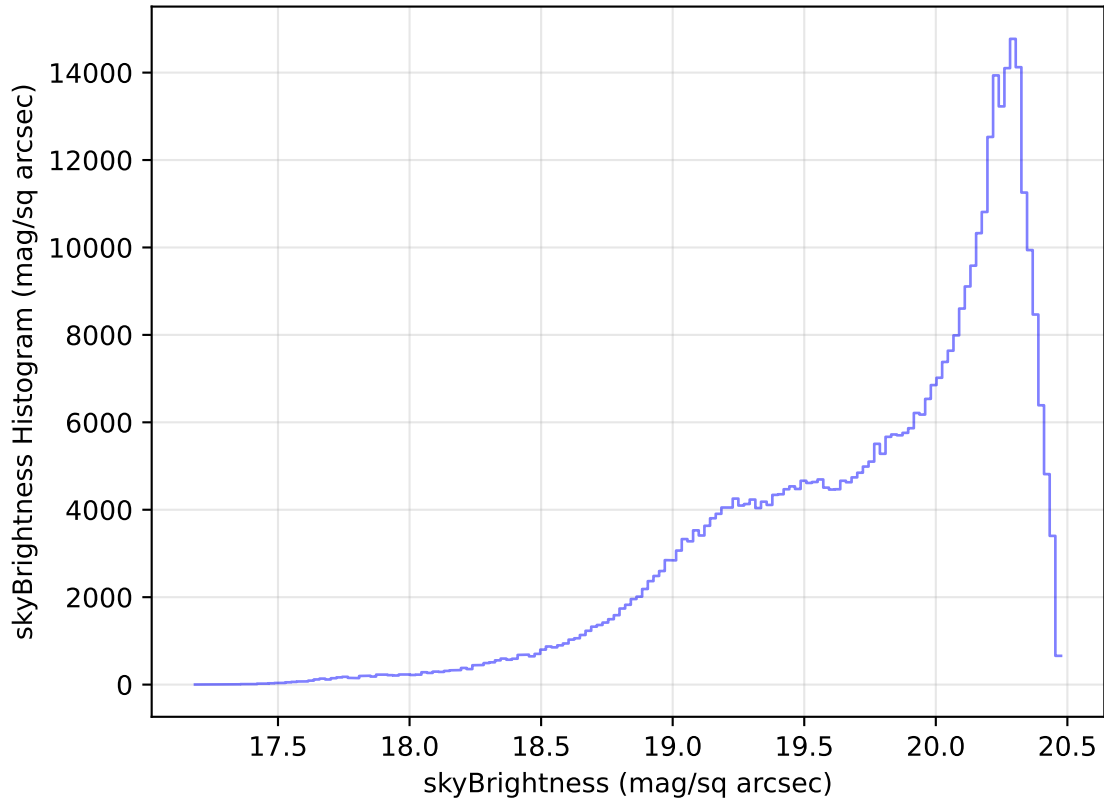
internal_u_expt45_nscale1.5v3.4_10yrs WFD i band: skyBrightness Histogram
