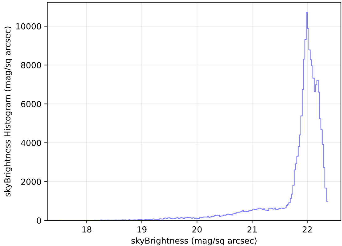
internal_u_expt45_nscale1.5v3.4_10yrs WFD g band: skyBrightness Histogram
