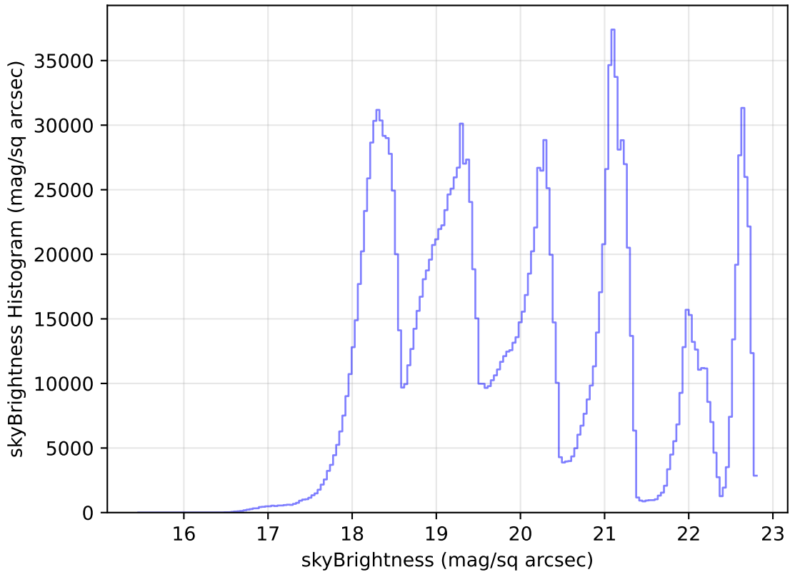
internal_u_expt45_nscale1.5v3.4_10yrs WFD all bands: skyBrightness Histogram
