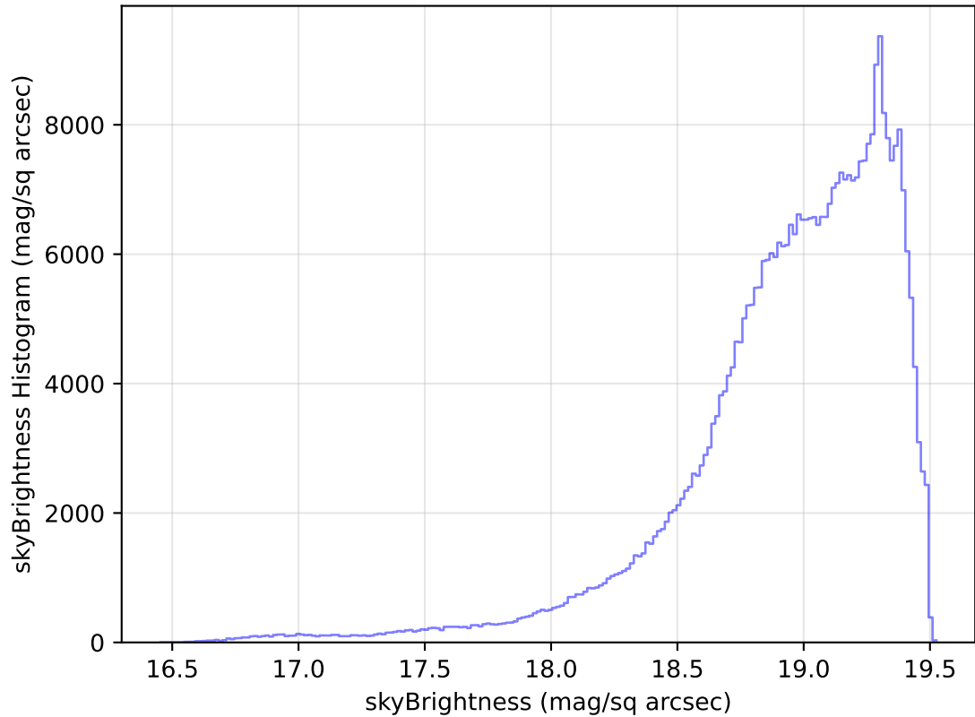
internal_u_expt45_nscale1.5v3.4_10yrs All sky z band: skyBrightness Histogram
