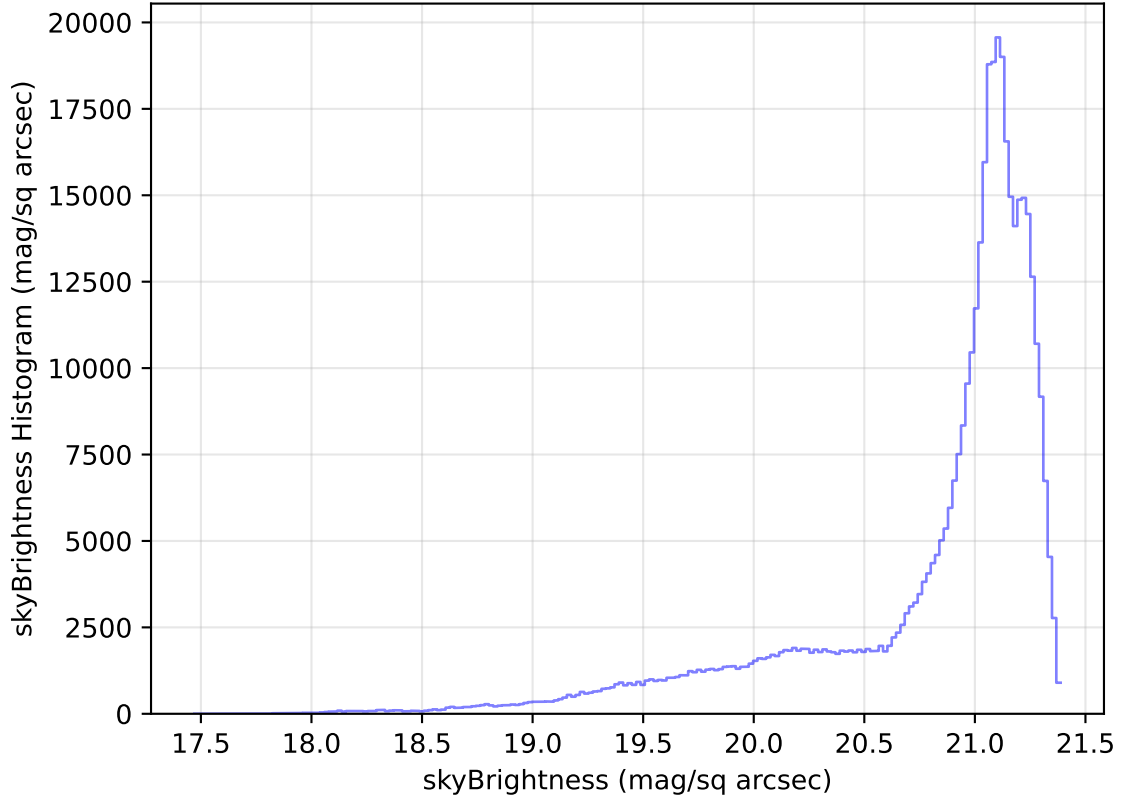
internal_u_expt45_nscale1.5v3.4_10yrs All sky r band: skyBrightness Histogram
