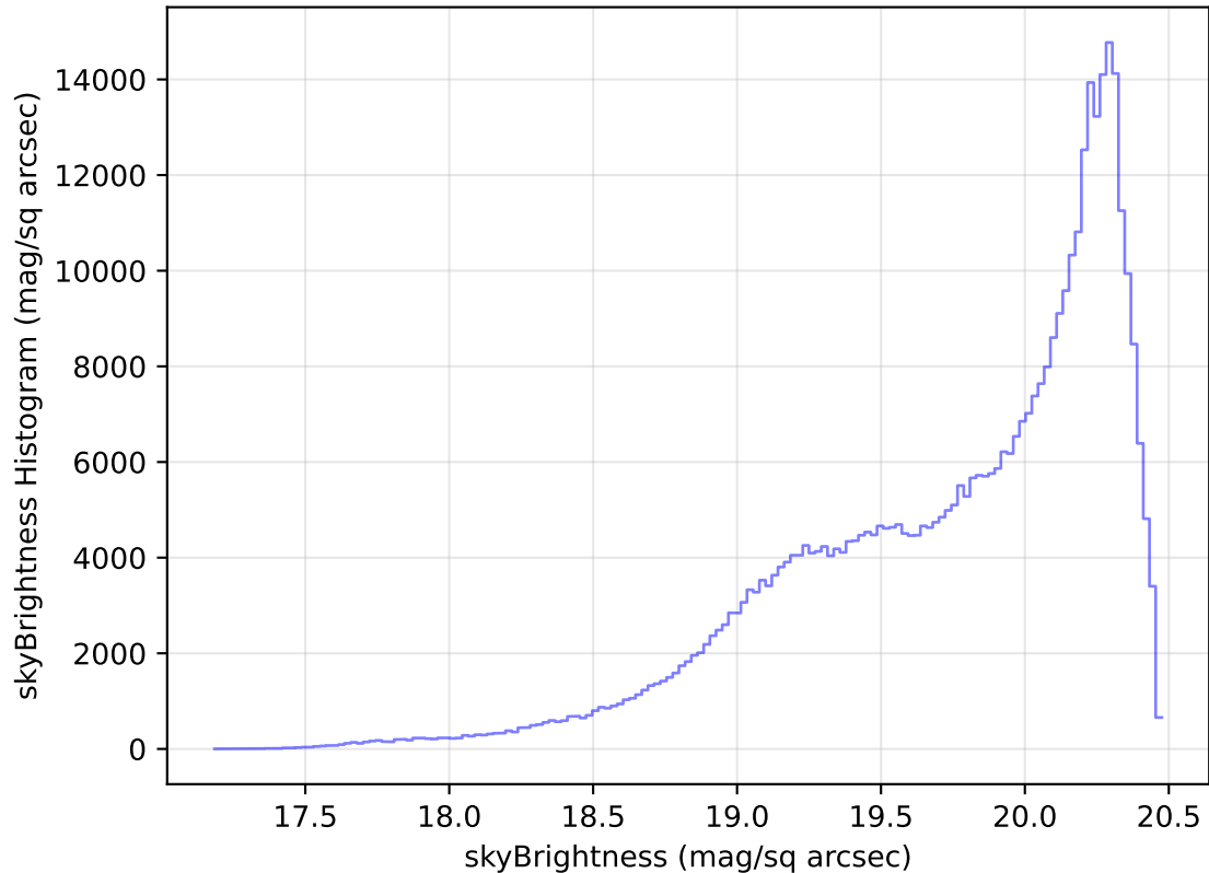
internal_u_expt45_nscale1.5v3.4_10yrs All sky i band: skyBrightness Histogram
