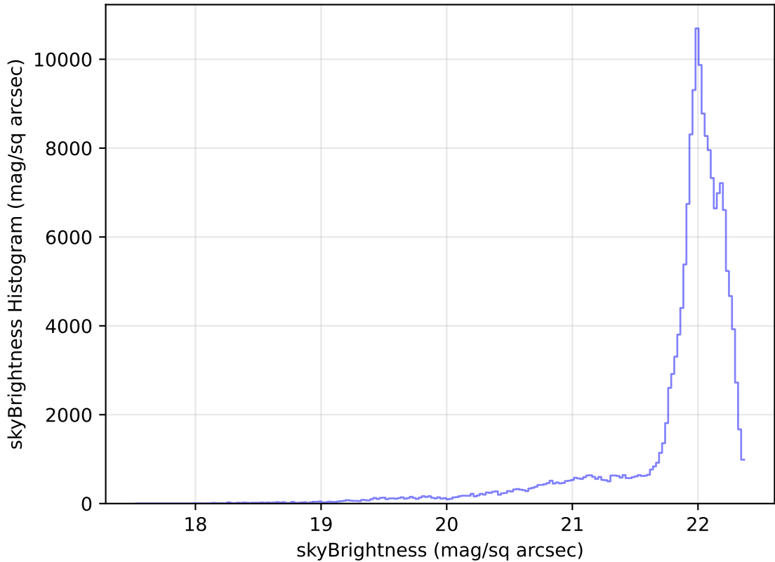
internal_u_expt45_nscale1.5v3.4_10yrs All sky g band: skyBrightness Histogram
