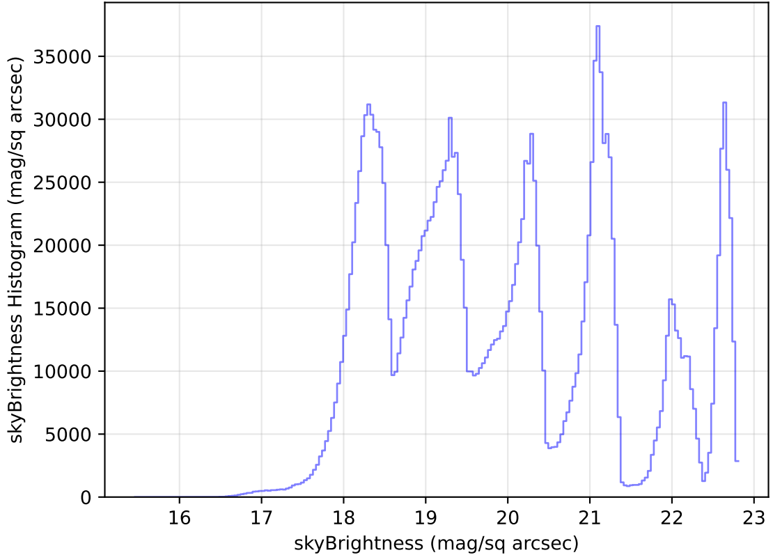
internal_u_expt45_nscale1.5v3.4_10yrs All sky all bands: skyBrightness Histogram
