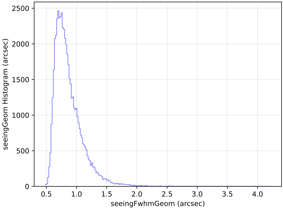
internal_u_expt45_nscale1.5v3.4_10yrs Yr 1 i band: seeingGeom Histogram
