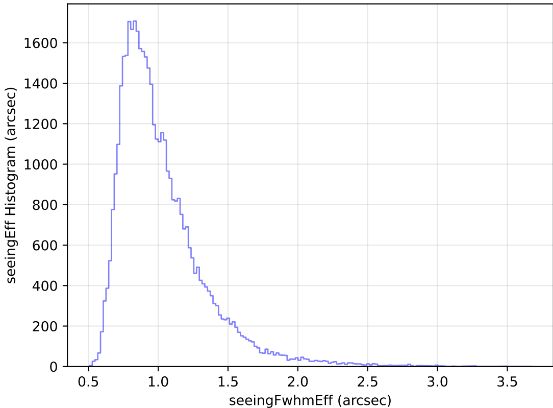
internal_u_expt45_nscale1.5v3.4_10yrs Yr 1 z band: seeingEff Histogram
