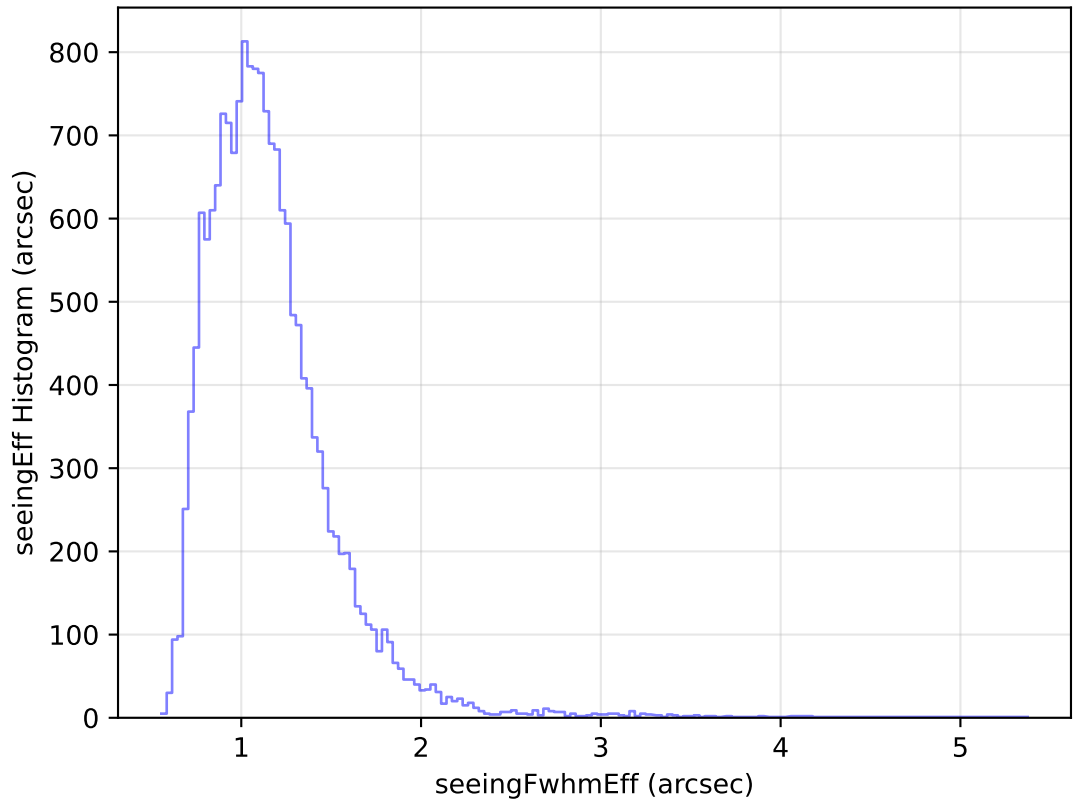
internal_u_expt45_nscale1.5v3.4_10yrs Yr 1 u band: seeingEff Histogram
