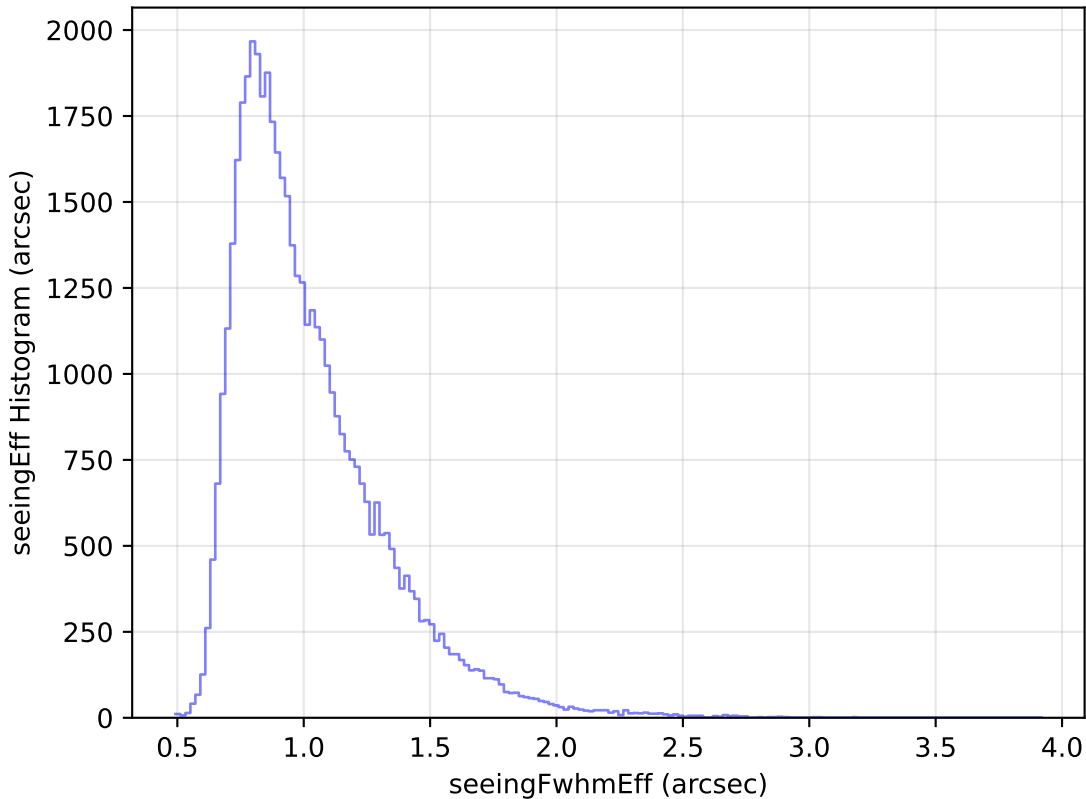
internal_u_expt45_nscale1.5v3.4_10yrs Yr 1 r band: seeingEff Histogram
