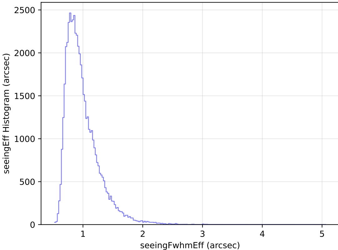
internal_u_expt45_nscale1.5v3.4_10yrs Yr 1 i band: seeingEff Histogram
