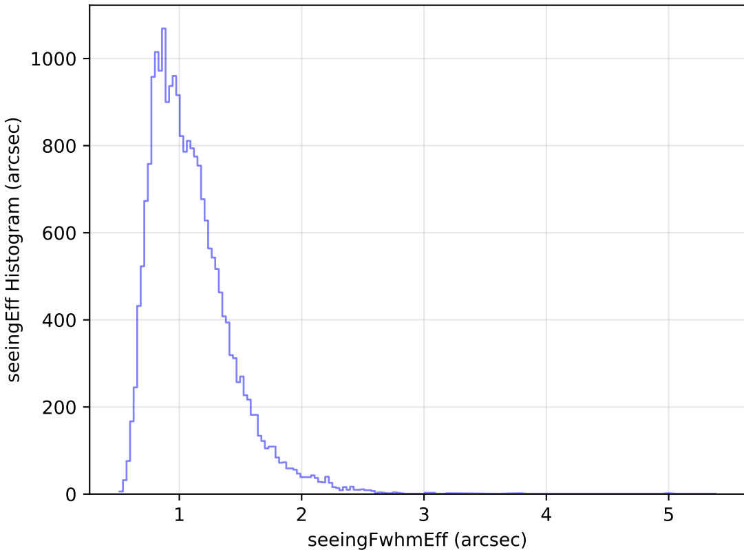
internal_u_expt45_nscale1.5v3.4_10yrs Yr 1 g band: seeingEff Histogram
