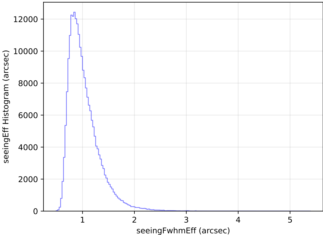
internal_u_expt45_nscale1.5v3.4_10yrs Yr 1 all bands: seeingEff Histogram
