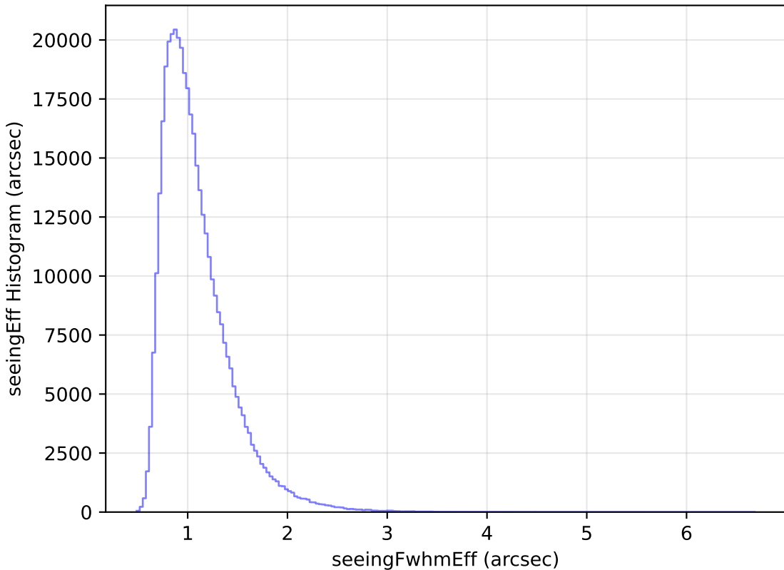
internal_u_expt45_nscale1.5v3.4_10yrs WFD z band: seeingEff Histogram
