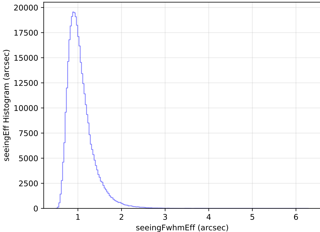
internal_u_expt45_nscale1.5v3.4_10yrs WFD y band: seeingEff Histogram
