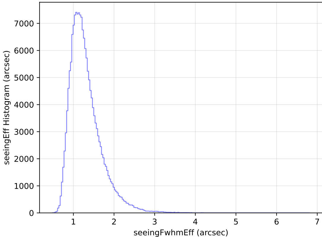
internal_u_expt45_nscale1.5v3.4_10yrs WFD u band: seeingEff Histogram
