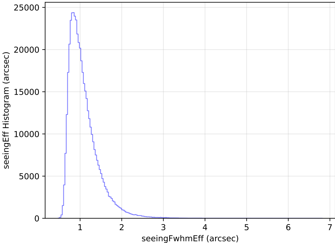
internal_u_expt45_nscale1.5v3.4_10yrs WFD i band: seeingEff Histogram
