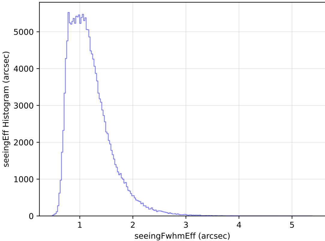
internal_u_expt45_nscale1.5v3.4_10yrs WFD g band: seeingEff Histogram
