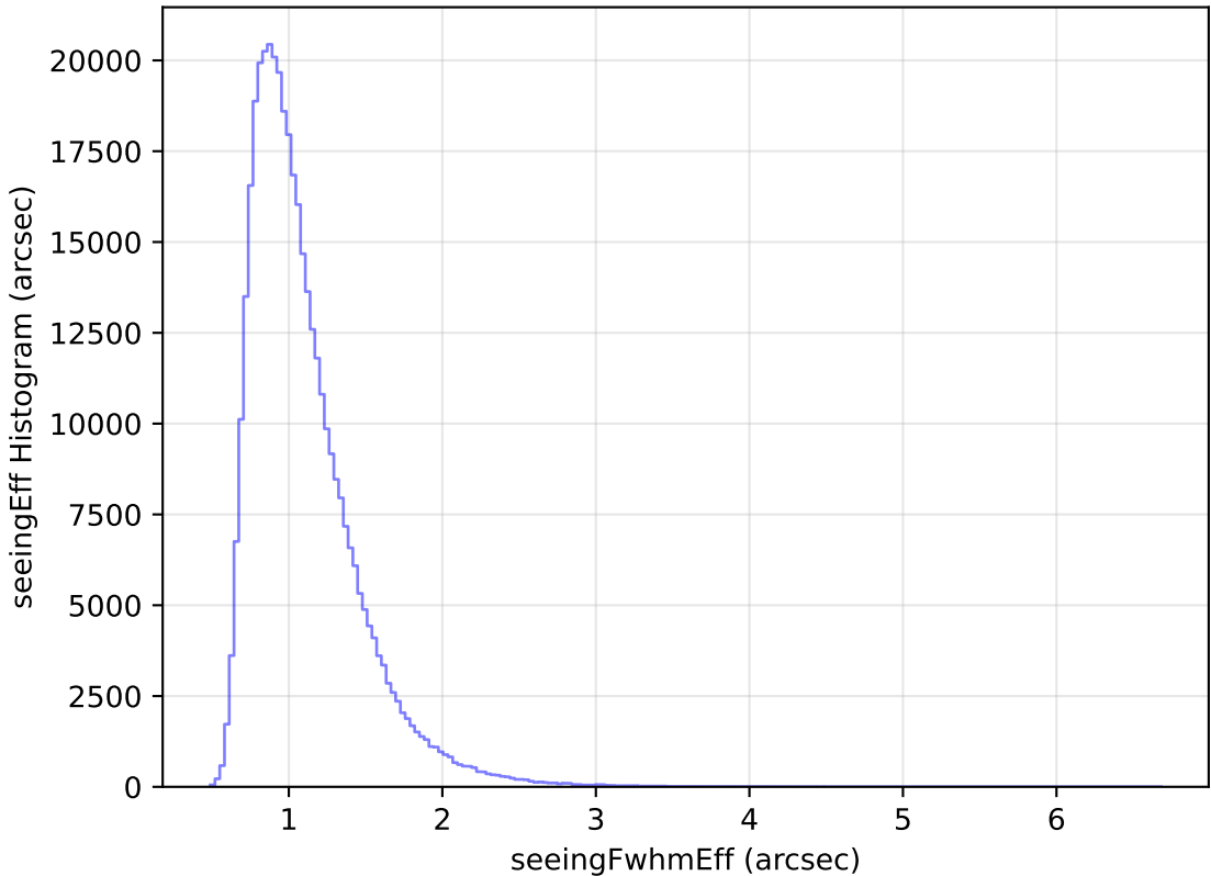
internal_u_expt45_nscale1.5v3.4_10yrs All sky z band: seeingEff Histogram
