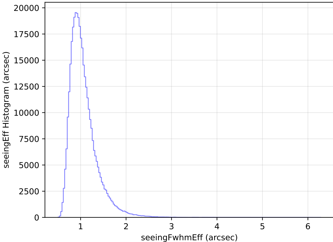
internal_u_expt45_nscale1.5v3.4_10yrs All sky y band: seeingEff Histogram
