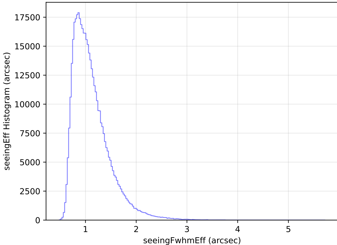
internal_u_expt45_nscale1.5v3.4_10yrs All sky r band: seeingEff Histogram
