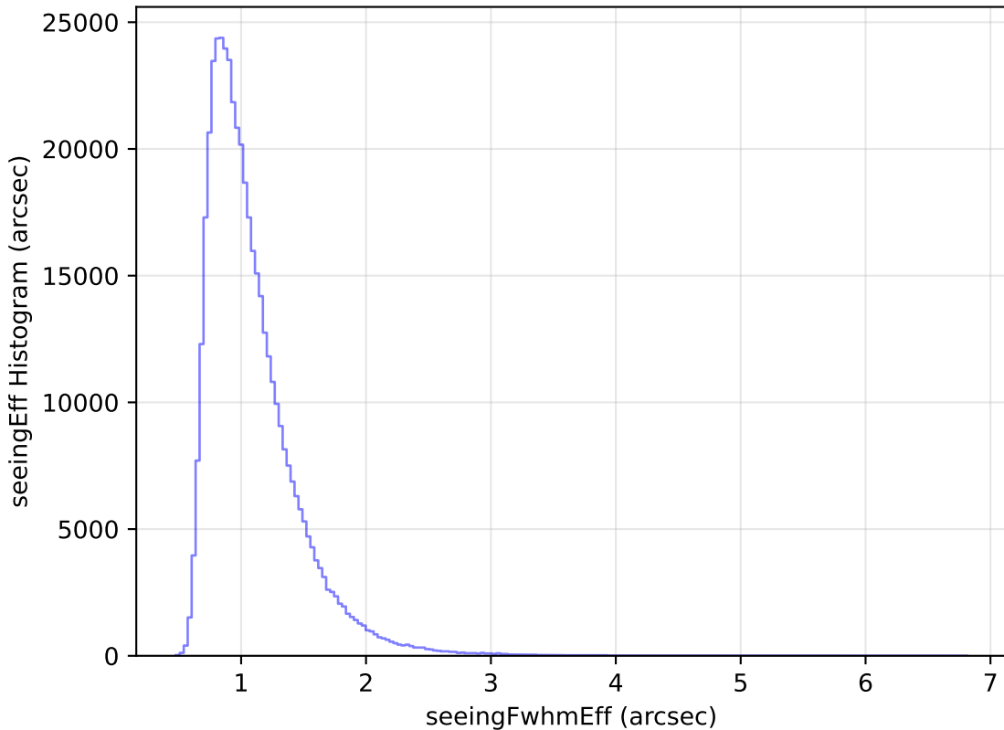
internal_u_expt45_nscale1.5v3.4_10yrs All sky i band: seeingEff Histogram
