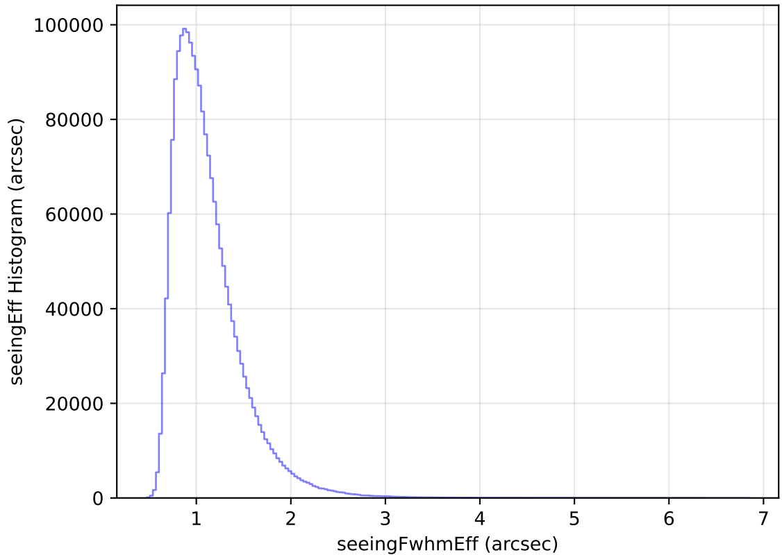
internal_u_expt45_nscale1.5v3.4_10yrs All sky all bands: seeingEff Histogram
