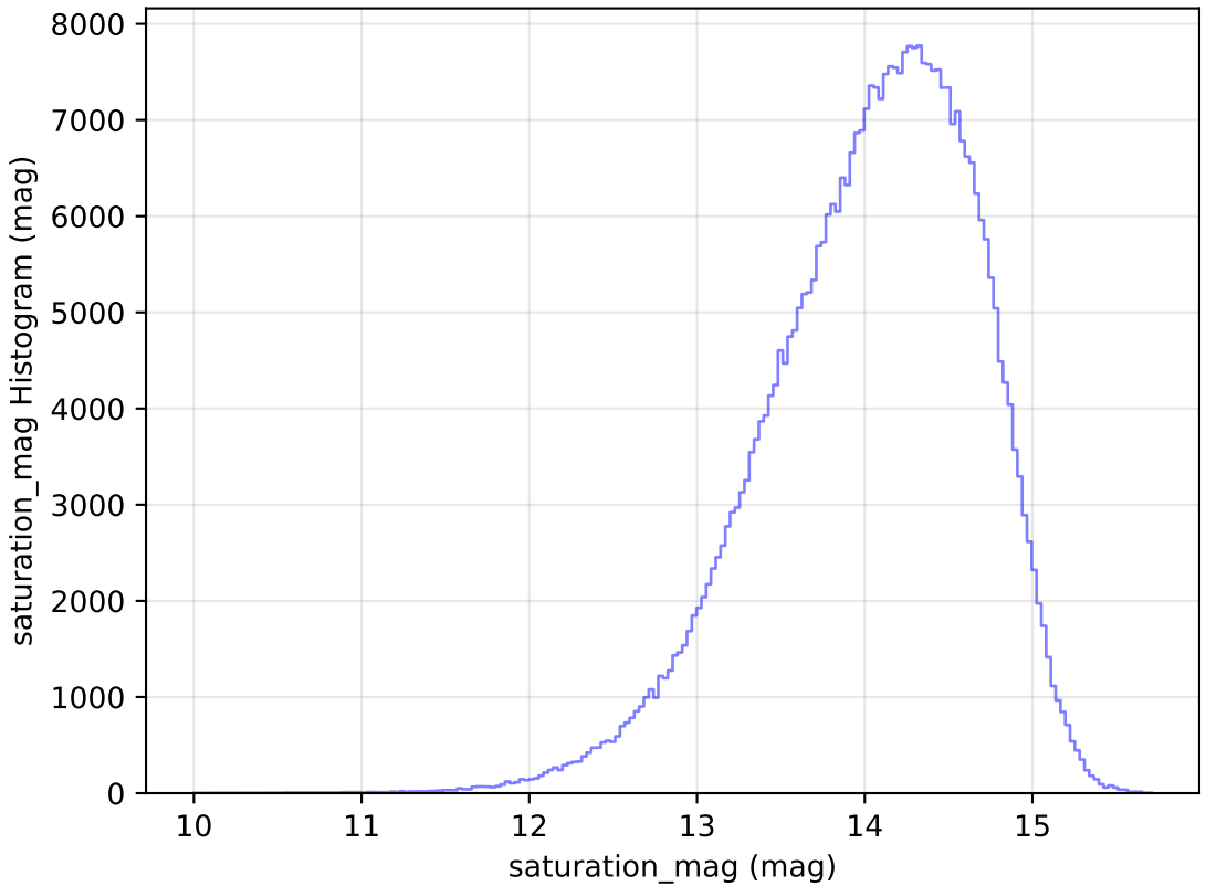
internal_u_expt45_nscale1.5v3.4_10yrs WFD z band: saturation_mag Histogram
