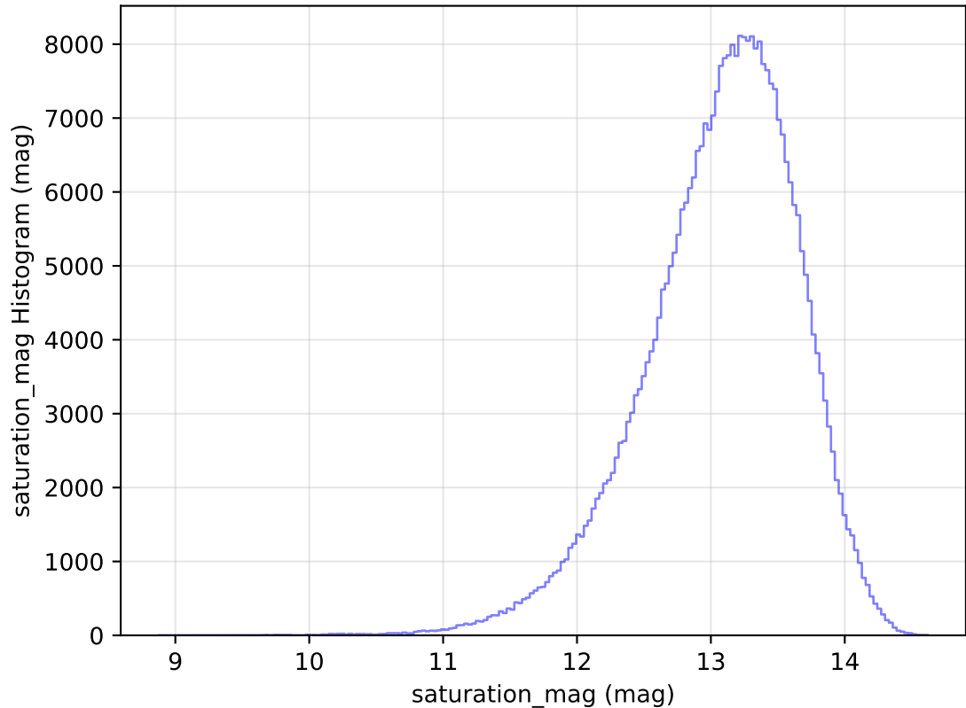
internal_u_expt45_nscale1.5v3.4_10yrs WFD y band: saturation_mag Histogram
