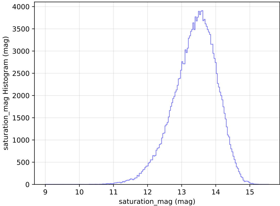
internal_u_expt45_nscale1.5v3.4_10yrs WFD u band: saturation_mag Histogram
