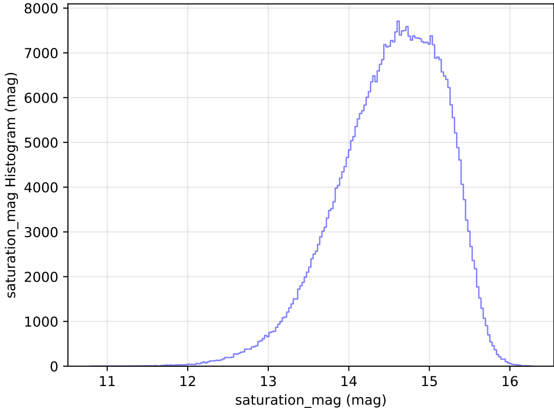
internal_u_expt45_nscale1.5v3.4_10yrs WFD r band: saturation_mag Histogram
