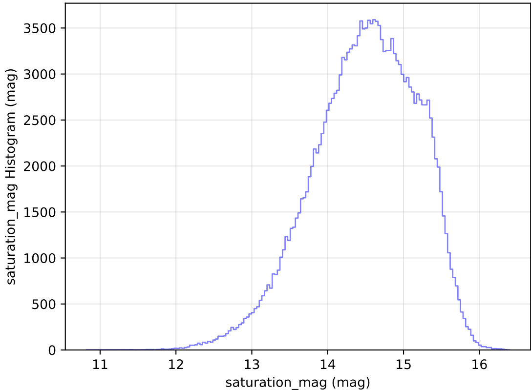
internal_u_expt45_nscale1.5v3.4_10yrs WFD g band: saturation_mag Histogram
