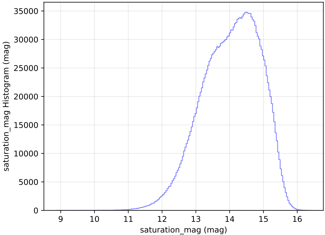
internal_u_expt45_nscale1.5v3.4_10yrs WFD all bands: saturation_mag Histogram
