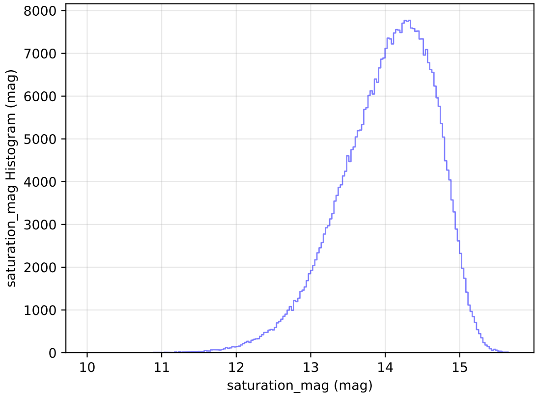
internal_u_expt45_nscale1.5v3.4_10yrs All sky z band: saturation_mag Histogram
