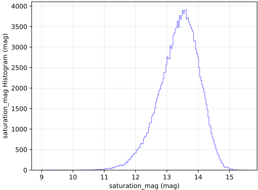
internal_u_expt45_nscale1.5v3.4_10yrs All sky u band: saturation_mag Histogram
