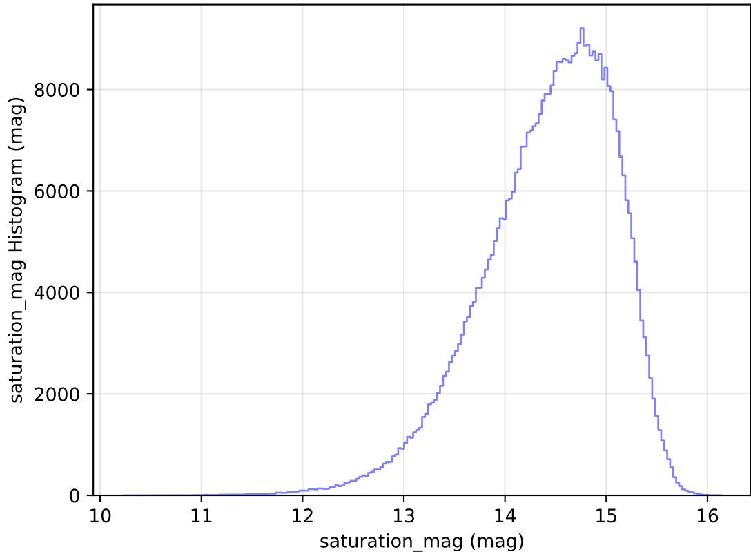
internal_u_expt45_nscale1.5v3.4_10yrs All sky i band: saturation_mag Histogram
