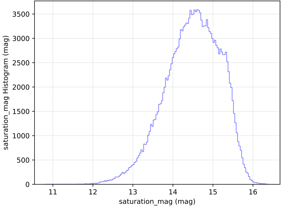
internal_u_expt45_nscale1.5v3.4_10yrs All sky g band: saturation_mag Histogram
