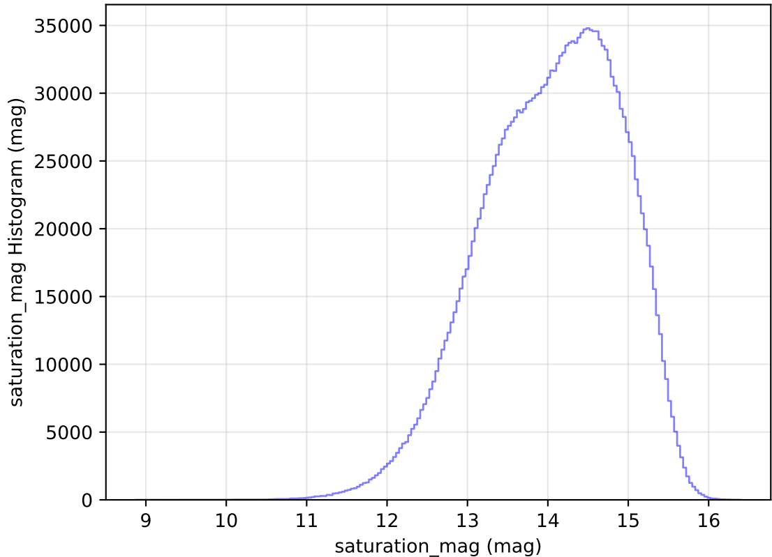
internal_u_expt45_nscale1.5v3.4_10yrs All sky all bands: saturation_mag Histogram
