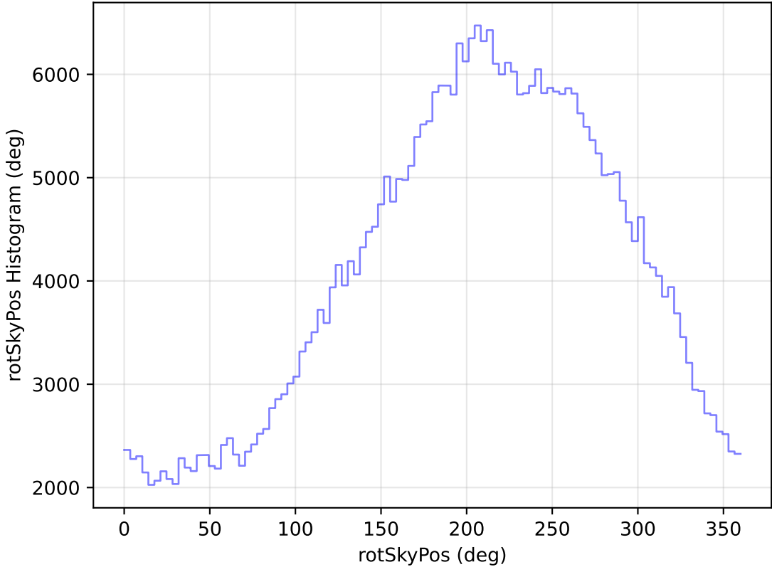
internal_u_expt45_nscale1.5v3.4_10yrs WFD z band: rotSkyPos Histogram
