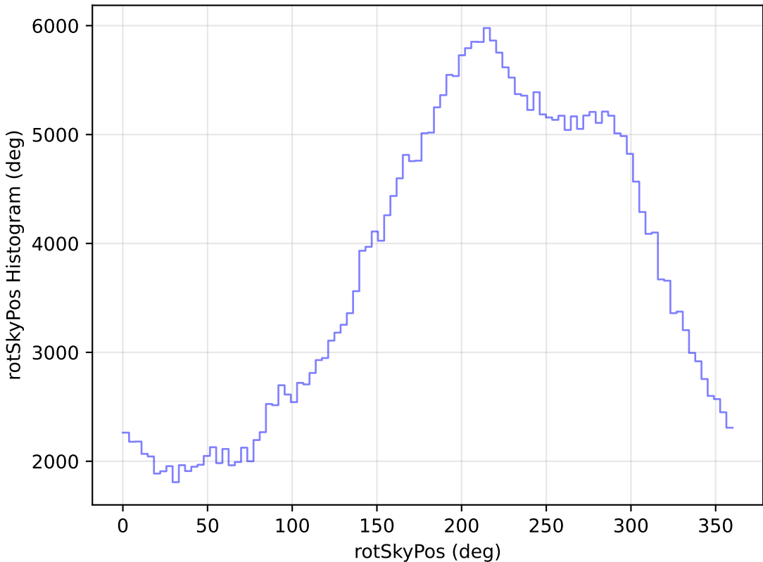
internal_u_expt45_nscale1.5v3.4_10yrs WFD y band: rotSkyPos Histogram
