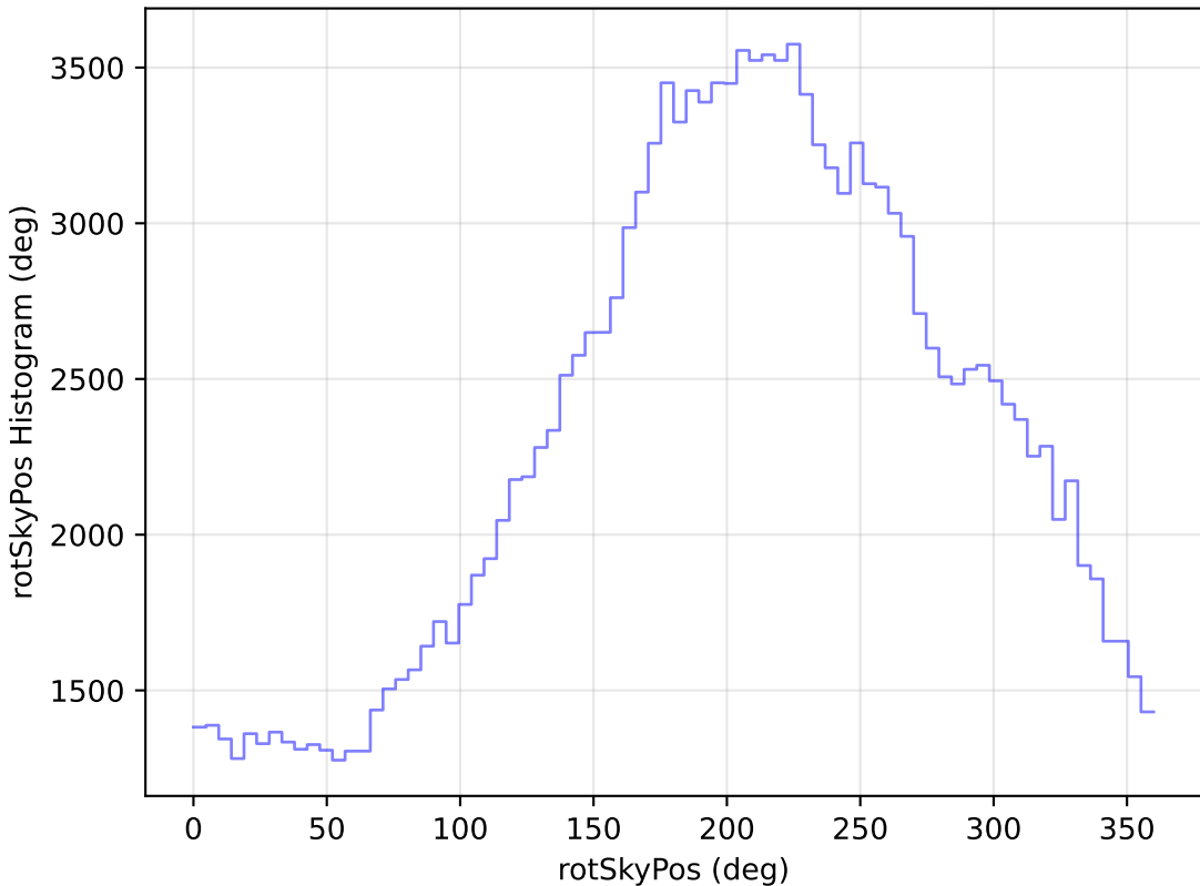
internal_u_expt45_nscale1.5v3.4_10yrs WFD u band: rotSkyPos Histogram
