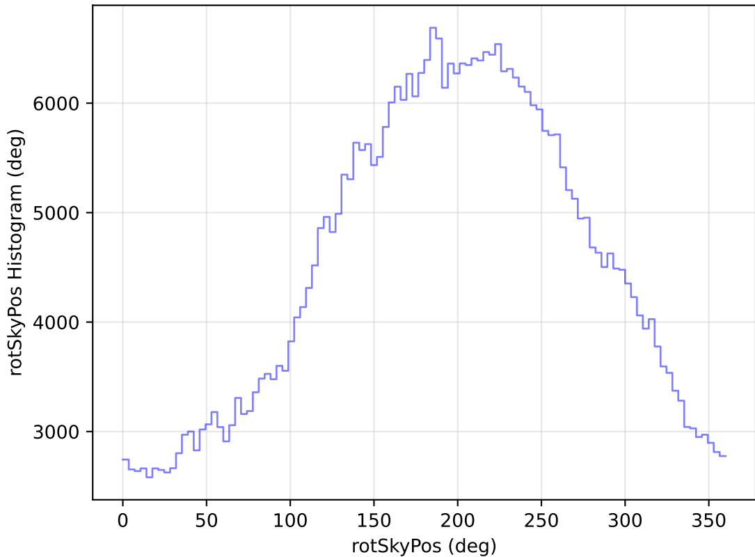
internal_u_expt45_nscale1.5v3.4_10yrs WFD r band: rotSkyPos Histogram
