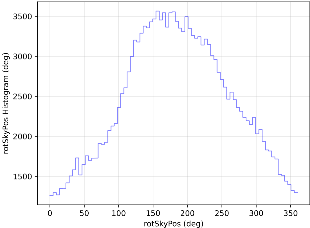
internal_u_expt45_nscale1.5v3.4_10yrs WFD g band: rotSkyPos Histogram
