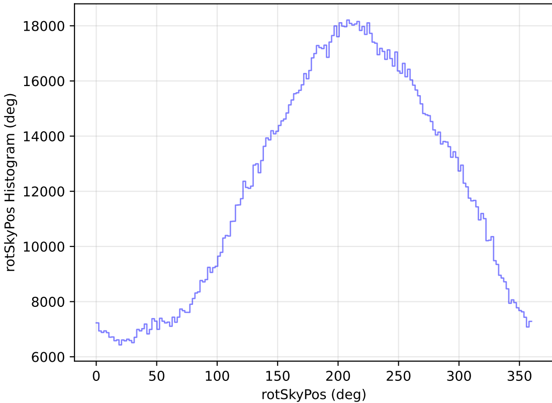
internal_u_expt45_nscale1.5v3.4_10yrs WFD all bands: rotSkyPos Histogram
