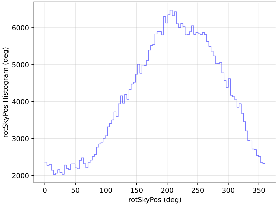
internal_u_expt45_nscale1.5v3.4_10yrs All sky z band: rotSkyPos Histogram
