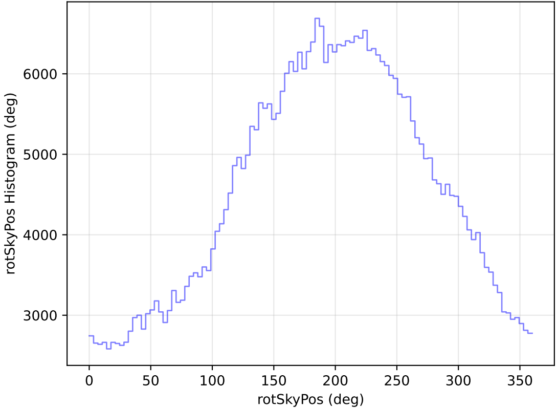
internal_u_expt45_nscale1.5v3.4_10yrs All sky r band: rotSkyPos Histogram
