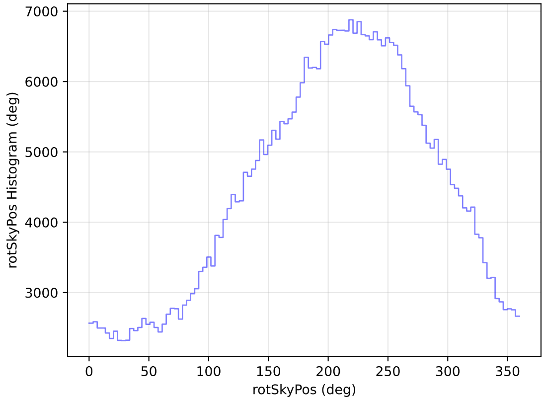
internal_u_expt45_nscale1.5v3.4_10yrs All sky i band: rotSkyPos Histogram
