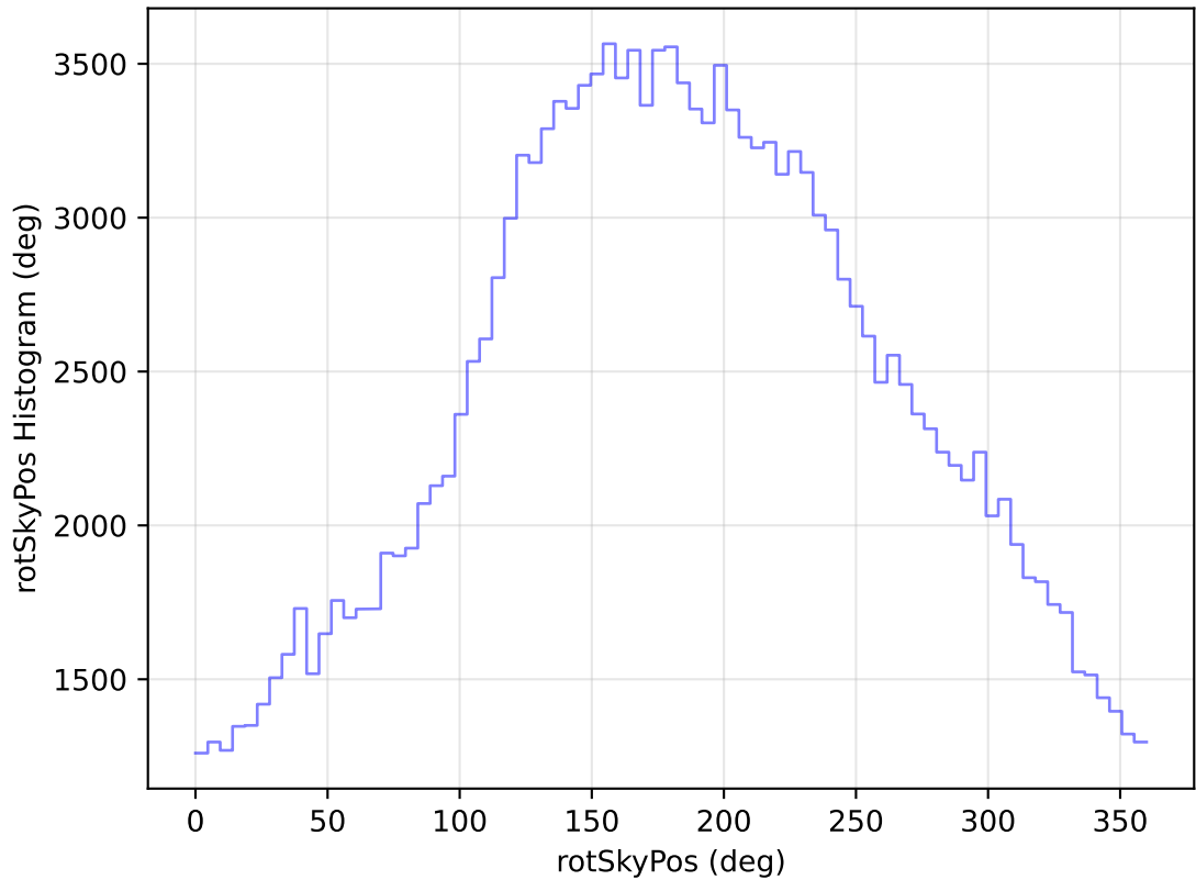
internal_u_expt45_nscale1.5v3.4_10yrs All sky g band: rotSkyPos Histogram
