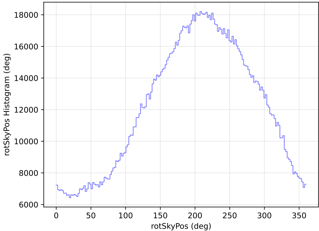
internal_u_expt45_nscale1.5v3.4_10yrs All sky all bands: rotSkyPos Histogram
