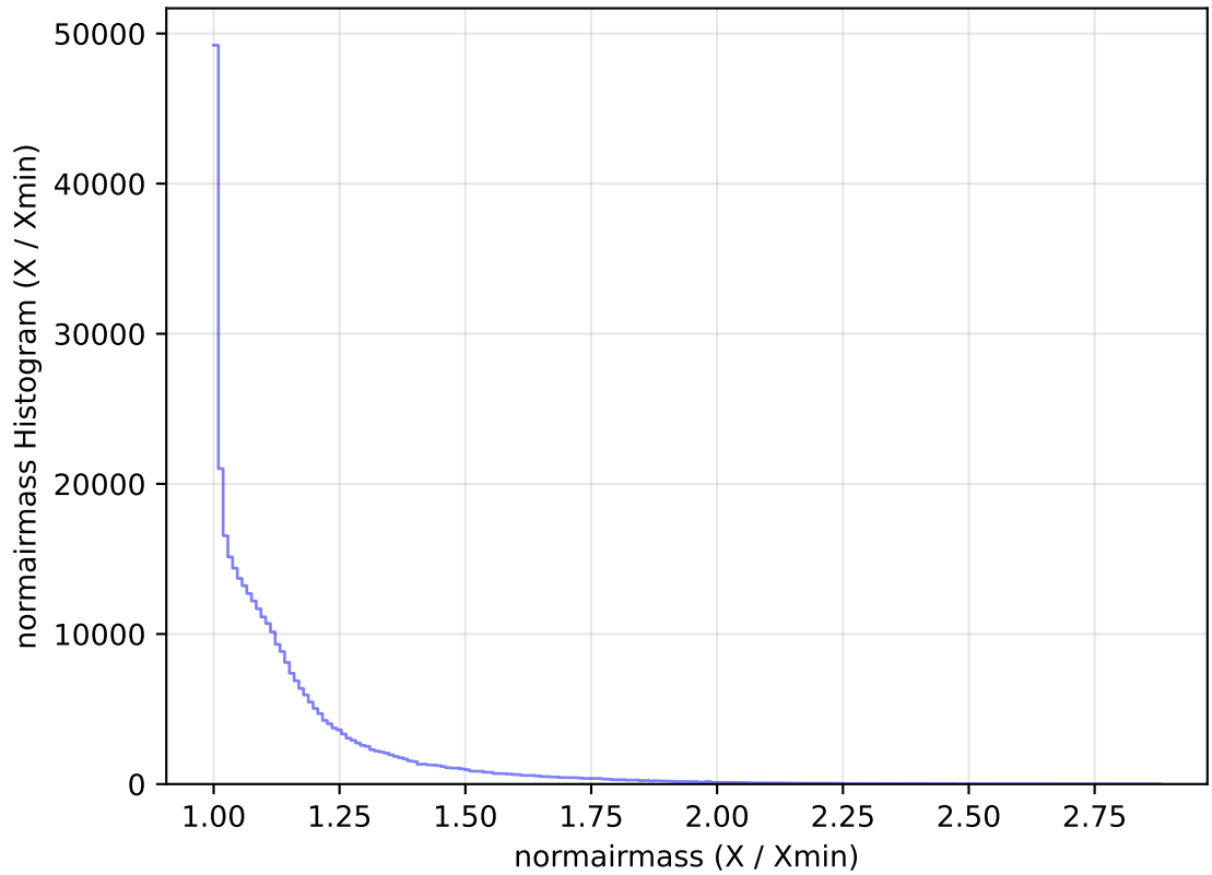
internal_u_expt45_nscale1.5v3.4_10yrs WFD y band: normairmass Histogram
