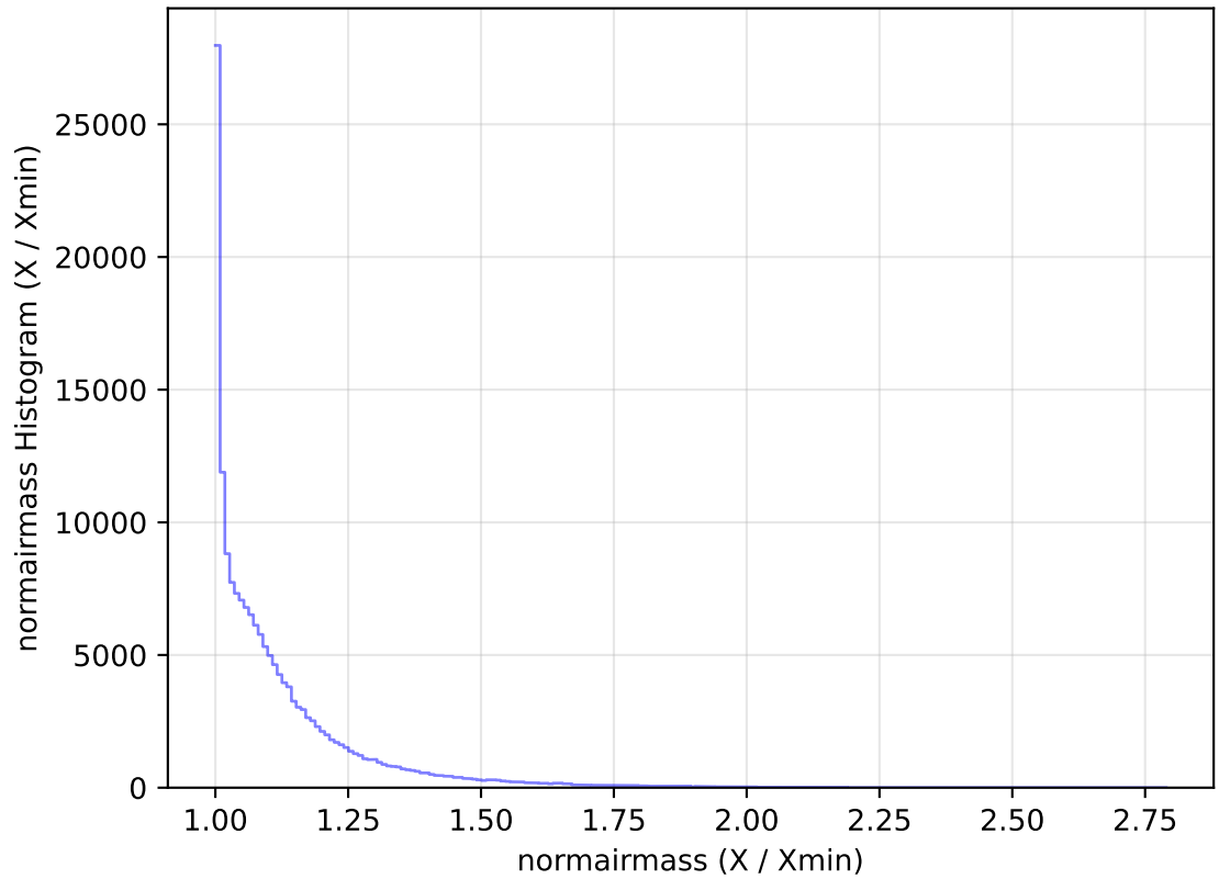
internal_u_expt45_nscale1.5v3.4_10yrs WFD u band: normairmass Histogram
