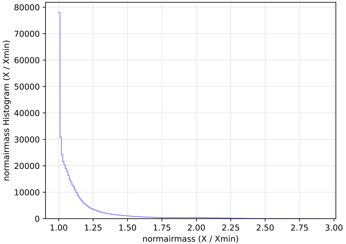
internal_u_expt45_nscale1.5v3.4_10yrs WFD r band: normairmass Histogram
